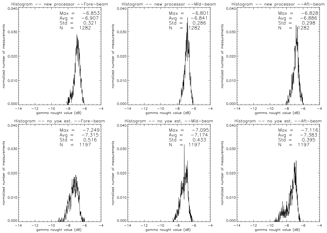
Figure 13. \gamma^0 histogram for data acquired during the ascending passes over the Brazilian rain forest for data acquired in zero-gyro mode. The upper graphs were obtained from products generated by the processor with yaw angle estimation while the lower graphs are from products produced by the processor without yaw angle estimation (yaw angle assumed equal to zero). The corresponding yaw angles made by the spacecraft are plotted in fig. 14.
