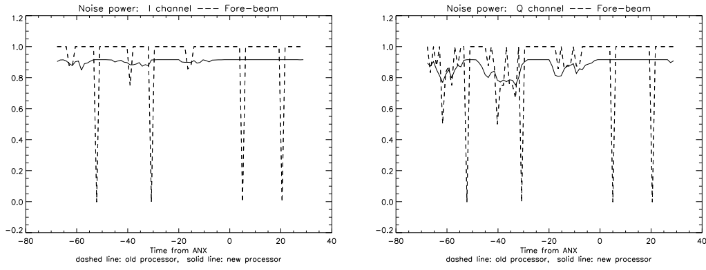
Figure 11. Typical along-track evolution of the per product noise power value for the old processor and for the new processor (left: in-phase (I) channel, right: in quadrature (Q) channel)
