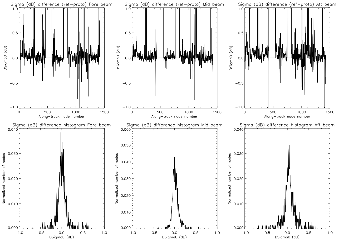
Figure 8. Upper graphs: along-track mid-swath nodes \sigma^0 difference between the old processor and the new one, for the three beams. Lower graphs: histogram of these differences.
