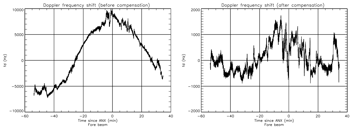
Figure 3. Illustration of the Doppler frequency shift correction on data acquired when the satellite was in fine pointing mode and received by the fore antenna. The along-track evolution of the mean signal spectrum center before and after residual Doppler frequency shift correction is shown respectively on the left and right graphs.
