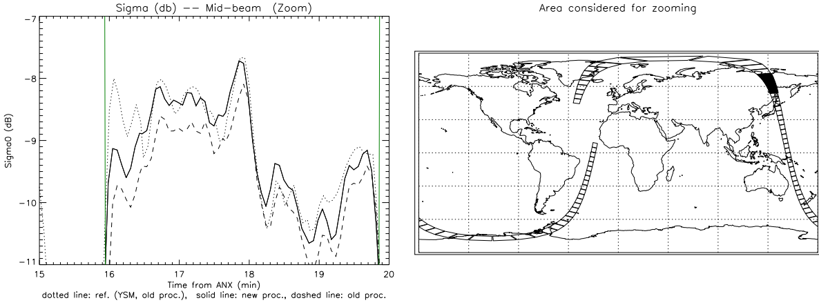
Figure 9. Left: comparison between the \sigma^0 value over land between the old and the new processor for a data set acquired in FPM mode. The nodes located between the two vertical lines are considered to be on earth. Right: orbit of which the data are extracted. The products filled black were considered for the comparison.
