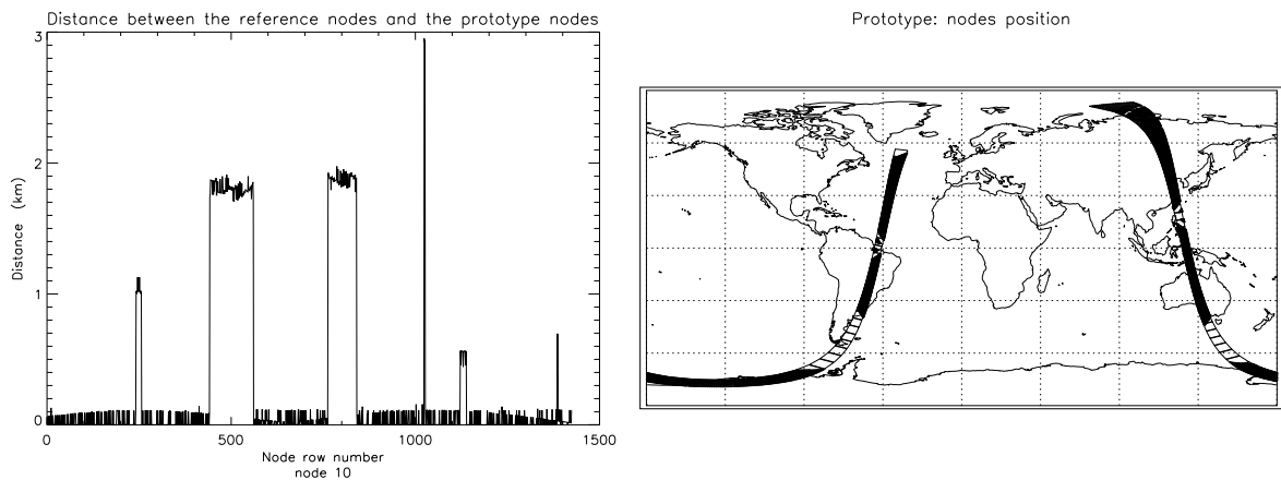
Figure 6. Left: great-circle distance between the mid-swath nodes generated by the old processor and the corresponding nodes generated by the new processor. The right graph shows the data gaps. The projected rectangles represent the products along the considered swath and the black dots inside the rectangles indicate valid nodes (nodes for which there were actually enough measurements).
