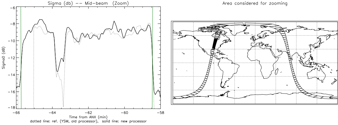
Figure 10. Left: comparison between the \sigma^0 value over land between the old and the new processor for a data set acquired in ZGM mode. Right: orbit of which the data are extracted. The products filled black were considered for the comparison.
