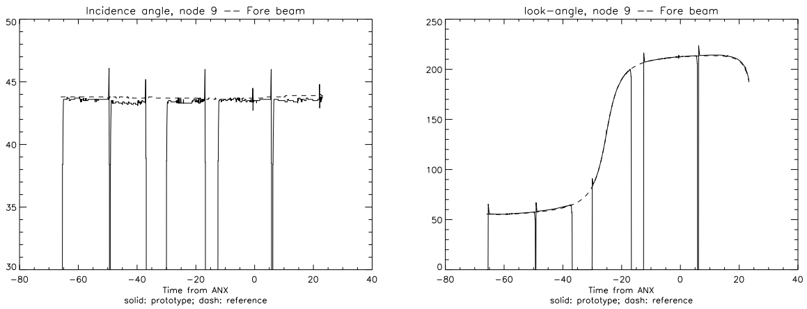
Figure 5. Incidence angle and look-angle at mid-swath. The solid line is the value obtained with the new processor while the dashed line is the value given by the old one.
