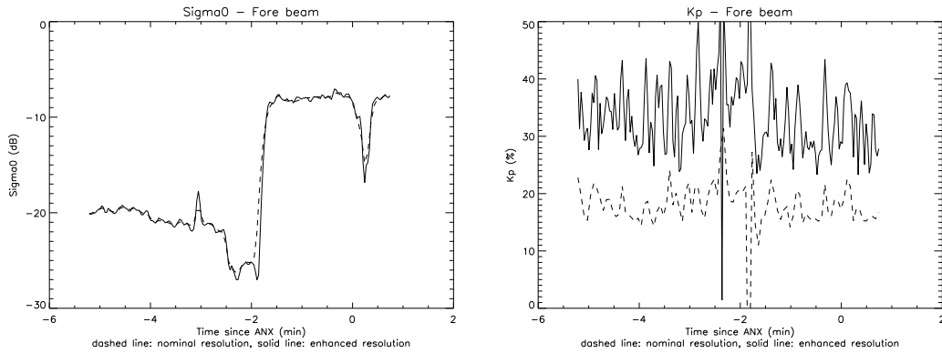
Figure 15. Comparison between the nominal resolution and the high-resolution products. The along-track evolution at mid-swath of respectively the \sigma^0 and the K_p are presented in the left and right graphs.
