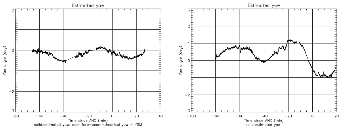
Figure 1. Along-track evolution of the yaw angle estimation for one orbit of data acquired when the spacecraft was in resp. yaw steering mode (left) and in zero-gyro mode (right). In yaw steering mode, the yaw angle should be zero while it can be arbitrary in ZGM.
