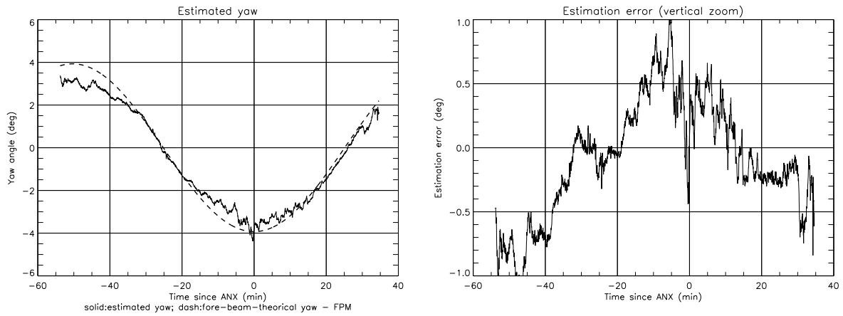
Figure 2. Along-track evolution of the yaw angle estimation for one orbit of data acquired when the spacecraft was in fine pointing mode (FPM). The dashed line in the left graphs shows the theoretical yaw angle, while the right graphs shows the estimation error (difference between the actual estimation and the theoretical prediction).
